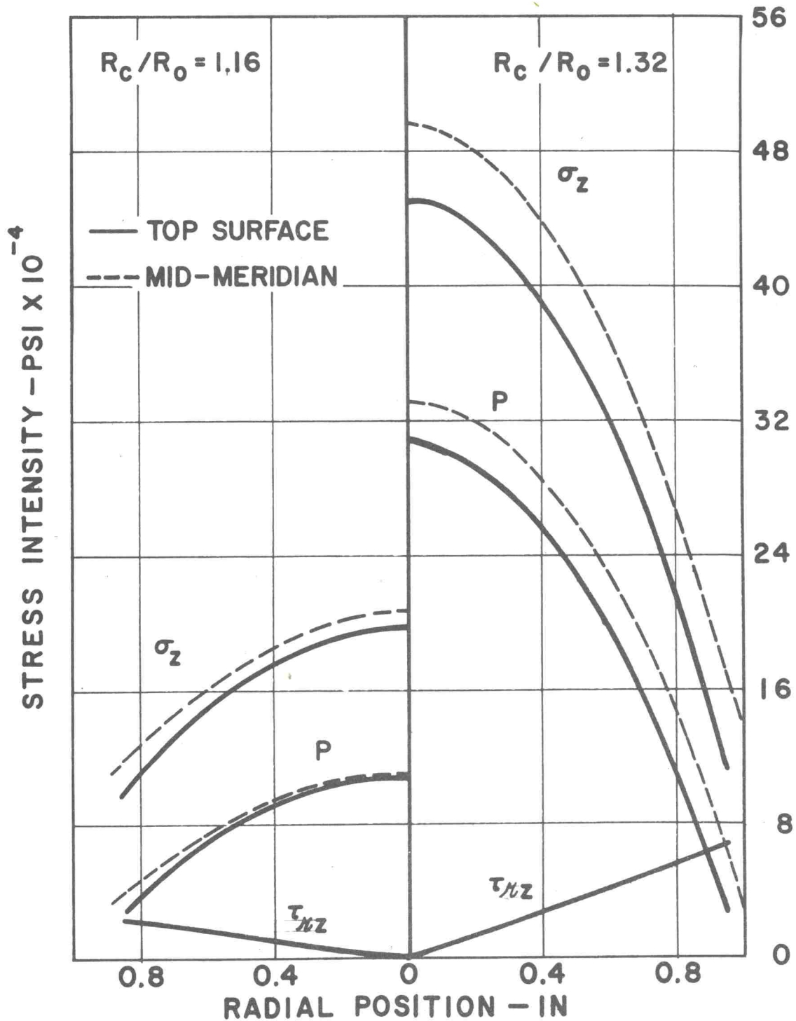
FIG. 8 STRESS DISTRIBUTION FOR 303 STAINLESS STEEL. CASE I-B
